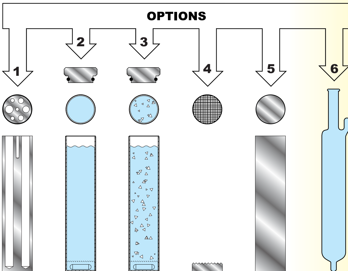
This schematic shows the six options available for the ISOCAL-6® range of calibration baths.
